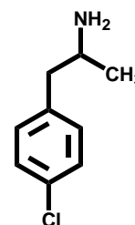
p -Chloroamphetamine (7)
