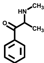
Methcathinone (6)
